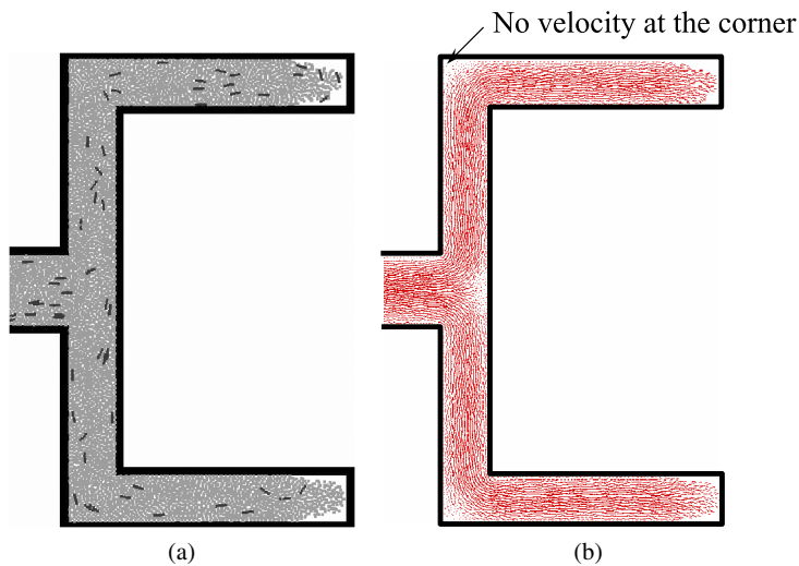
Figure 7. Simulated results of injection into a mold with a corner. (a) Particle motion. (b) Velocity distribution. This figure is published in color in the online version.
