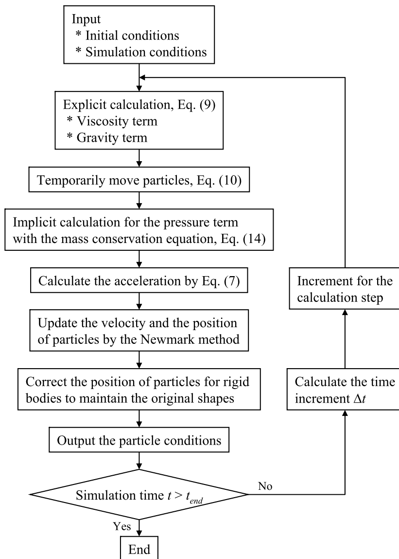
Figure 3. Flowchart of the simulation.
