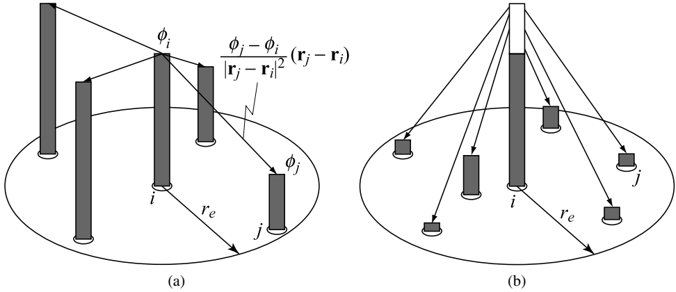
Figure 2. Particle-interaction models for differential operators. (a) Gradient model. (b) Laplacian model.
