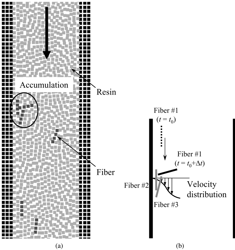
Figure 6. Fiber accumulation near the wall. Fibers #2 and #3 near the wall almost stopped during the small time increment \Delta t . (a) Particle motion. (b) Schematic.
