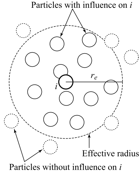
Figure 1. Schematic diagram of the interaction between neighboring particles.
