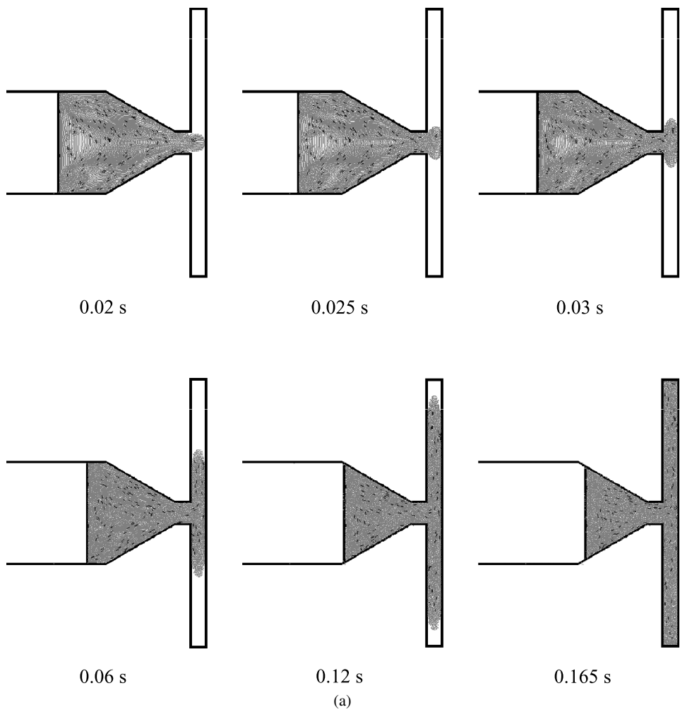
Figure 5. Simulated results of injection into the plate mold. (a) Particle motion. (b) Velocity distribution. This figure is published in color in the online version.
