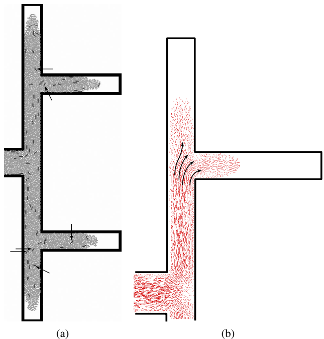
Figure 8. Disturbed fiber orientation near a branch. Arrows in (a) show the fibers inclined from the flow direction after passing the branches. (a) Particle motion. (b) Velocity distribution. This figure is published in color in the online version.
