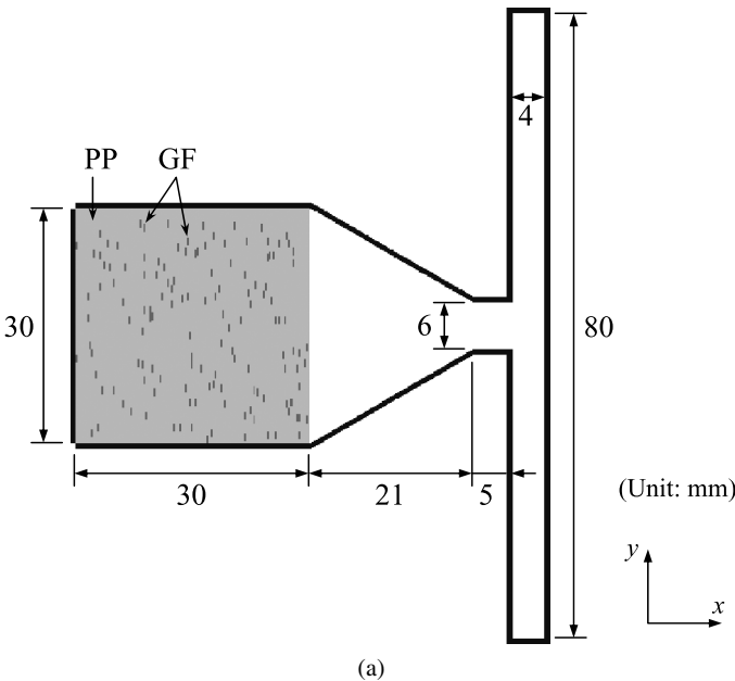
Figure 4. Particle model for injection molding with (a) a plate mold, (b) a mold with a corner and (c) a mold with a branch. PP and GF denote polypropylene and glass fiber.
